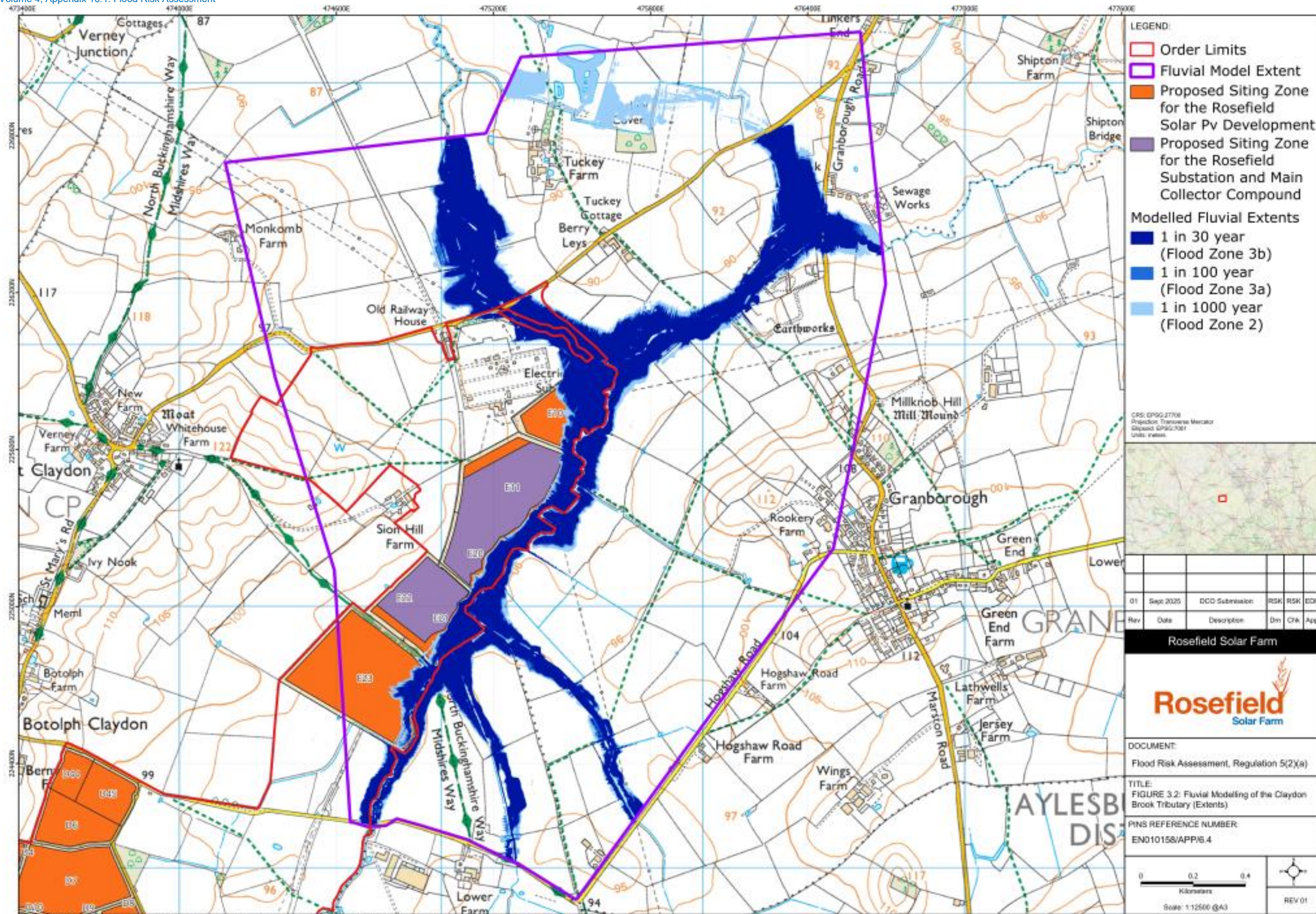
Figure 3.2: Fluvial Modelling of Claydon Brook Tributary
