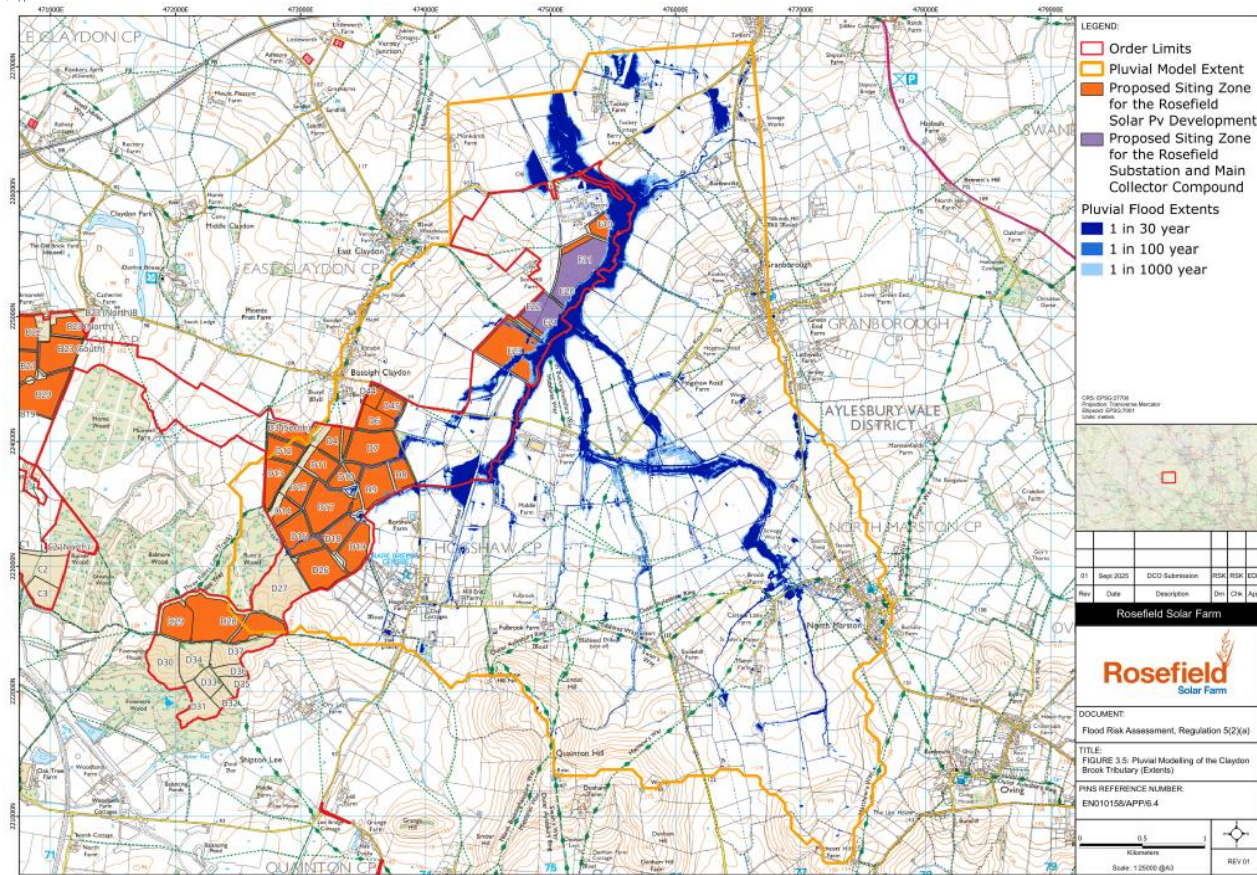
Figure 3.5: Pluvial Modelling of Claydon Brook Tributary
